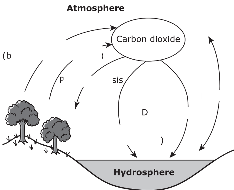
Figure 1: Carbon Cycle between Atmosphere and Hydrosphere
