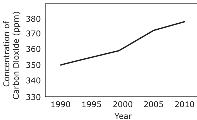
Figure 4: Concentration of Atmospheric Carbon Dioxide
